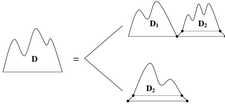
Figure 6: The last return decomposition of a Dyck path.
