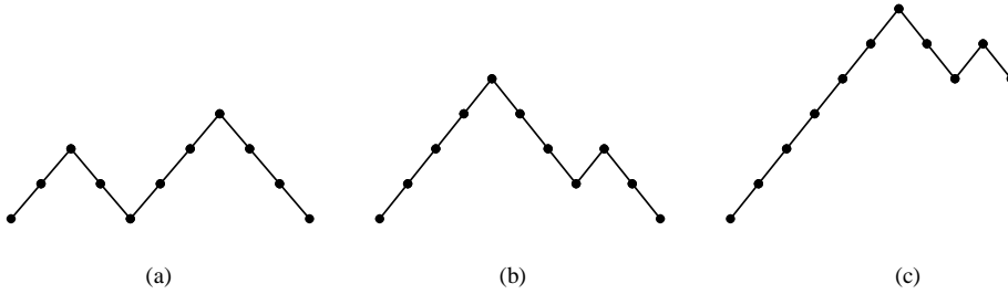
Figure 5: The Dyck prefixes associated with the permutations (a) 91068743512 \in K_{10}(123) , (b) 71096835214 \in CK_{10}(123) , and (c) 51094837216 \in G_{10}(123) .
