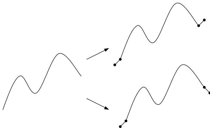
Figure 7: The generation of two new Dyck prefixes of length 2n from a Dyck prefix of length 2n - 2 .
