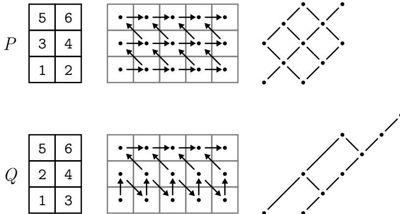
Figure 23: The tableaux P and Q and their corresponding Hasse diagrams.
