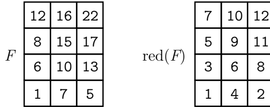
Figure 2: An example of F \in \mathcal{F}_{3,4} and red(F) .
