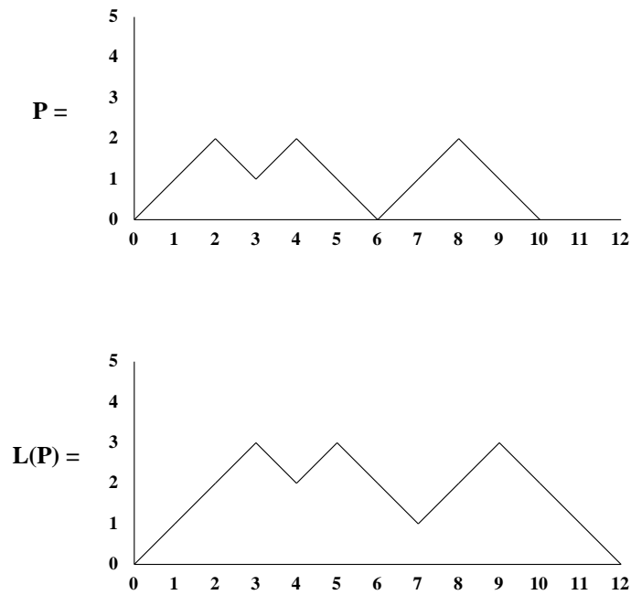
Figure 2: The lifting of a Dyck path.
